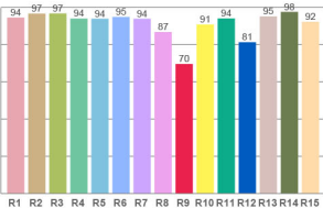
CRI: 93.9 (R1-R8)
